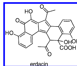
Figure 2. Erdacin is produced by heterologous expression of the eDNA-derived Erd gene cluster in S. albus .
