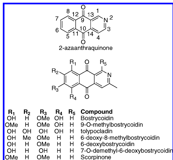
Figure 1. Known 2-azaanthraquinones from fungi and lichens.
