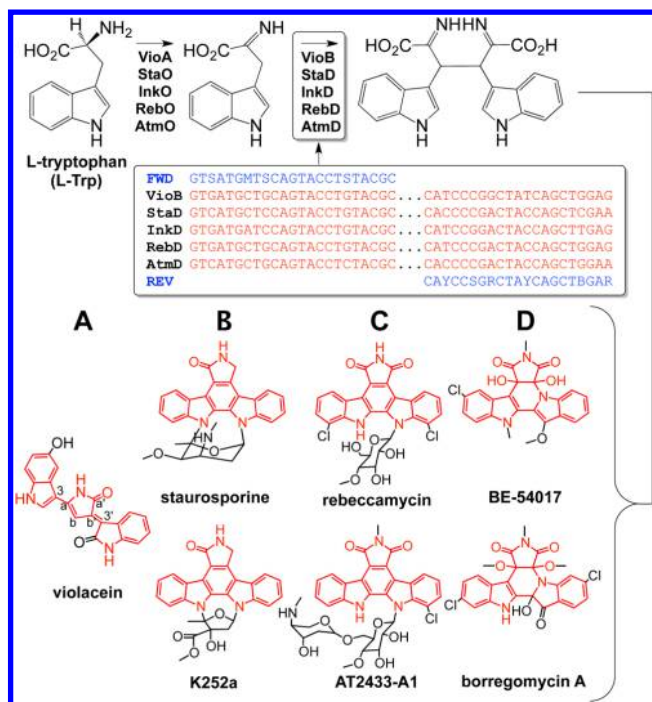
Figure 1. Conserved biosynthetic steps by IPA-imine synthase and CPA synthase that initiate the production of known bacterial TDs with varied substructures (A–D). Degenerate PCR primers (A–D). Degenerate PCR primers were designed based on conserved regions of CPA synthase genes.
