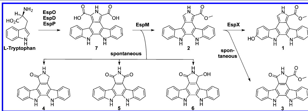
Figure 5. Proposed biosynthetic scheme for the erdasporines. Key steps include methylation of the dicarboxy-indolocarbazole (7) by EspM to generate 2 and the hydroxylation of 2 by EspX to give 1.
