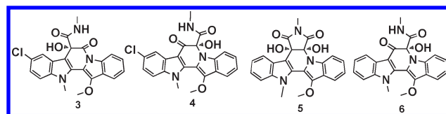
Figure 4. Minor compounds isolated from the culture broth of S. albus transformed with the abe gene cluster.
